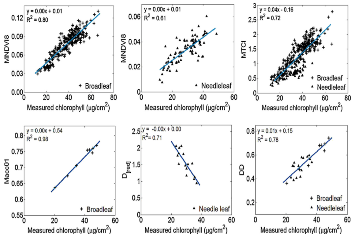
Fig. 9 – Relationship between reflectance indices (MNDV18, MTCI, Macc01, D, DD) and leaf chlorophyll content (broad or needle site). From Croft et al. (2014).
