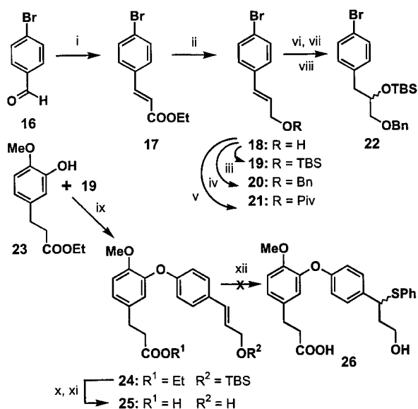
Scheme 2. Attempts to prepare seco acid 26 . Reagents and conditions: i) 1.2 equiv \text{Ph}_3\text{P}=\text{CHCOOEt} , benzene, 25^\circ\text{C} , 30 min, 93%; ii) 2.1 equiv DIBAL, \text{CH}_2\text{Cl}_2 , -78^\circ\text{C} , 20 min, 97%; iii) 1.2 equiv TBSCl, 1.4 equiv imidazole, DMF, 25^\circ\text{C} , 3 h, 97%; iv) 1.1 equiv NaH, THF, 0 \rightarrow 25^\circ\text{C} , 30 min, then 1.2 equiv BnBr, cat. \text{Bu}_4\text{NI} , 3 h, 25^\circ\text{C} , 94%; v) 1.7 equiv PivCl, pyridine, DMF, 0 \rightarrow 25^\circ\text{C} , 6 h, 87%; vi) 1.5 equiv m -CPBA, \text{CH}_2\text{Cl}_2 , 25^\circ\text{C} , 4 h, 82%; vii) 1.1 equiv DIBAL, toluene, 0^\circ\text{C} , 30 min, 86%; viii) 1.1 equiv TBSCl, 1.3 equiv imidazole, DMF, 25^\circ\text{C} , 3 h, 97%; ix) 2 equiv \text{CuBr} \cdot \text{Me}_2\text{S} , 6 equiv \text{K}_2\text{CO}_3 , pyridine, 6 h, 140^\circ\text{C} , 78%; x) 2.5 equiv TBAF, THF, 25^\circ\text{C} , 3 h, 96%; xi) \text{LiOH} \cdot 3\text{N}:\text{THF}:\text{MeOH} \ 1:1:1 , 0 \rightarrow 25^\circ\text{C} , 2 h, 92%; xii) 3 equiv PhSH, AcOEt, 25^\circ\text{C} , 5 h. TBS = tert -butyldimethylsilyl, Bn = benzyl, Piv = pivaloyl, TBAF = tetrabutylammonium fluoride.
