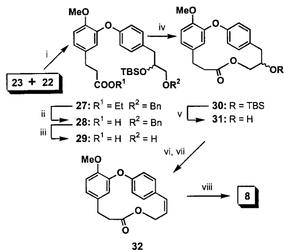
Scheme 3. Formal synthesis of combretastatin D-2 ( 8 ). Reagents and conditions: i) 2 equiv \text{CuBr} \cdot \text{Me}_2\text{S} , 0.7 equiv 22 , 6 equiv \text{K}_2\text{CO}_3 , pyridine, 6 h, 140^\circ\text{C} , 92%; ii) \text{LiOH} \cdot 3\text{N}:\text{THF}:\text{MeOH} \ 1:1:1 , 0 \rightarrow 25^\circ\text{C} , 2 h, 94%; iii) \text{H}_2 , Pd/C 10%, AcOEt, 25^\circ\text{C} , 4 h, 100%; iv) 9 equiv DEAD, 8.8 equiv \text{Ph}_3\text{P} , toluene 2.5 mm final concentration, 45^\circ\text{C} , 7 h addition, 91%; v) 1.2 equiv TBAF, THF, 25^\circ\text{C} , 0.5 h, 94%; vi) 2 equiv \text{I}_2 , 2 equiv \text{Ph}_3\text{P} , 3 equiv imidazole, toluene, 80^\circ\text{C} , 30 min, 95%; vii) 10 equiv KF, DMSO 0.15 M, 115^\circ\text{C} , 4 h, 87%; viii) 1 equiv \text{BI}_3 , 1.2 equiv N,N -dimethylaniline, benzene, 0 \rightarrow 25^\circ\text{C} , 17%.
