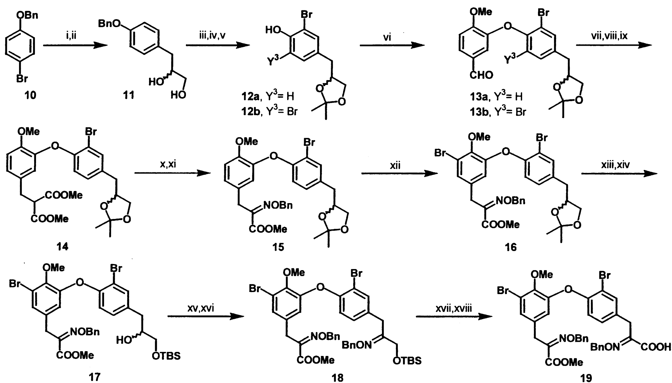
Scheme 2. Synthesis of the eastern segment of bastadins 7, 10, 12, 14 and 15. Reagents and conditions: (i) Mg, THF, reflux, allyl bromide, 93%; (ii) K 2 OsO 2 (OH) 2 , tert -BuOH/H 2 O, K 3 Fe(CN) 6 , K 2 CO 3 , rt, 99%; (iii) 2,2-dimethoxypropane, acetone, PPTS, rt, 95%; (iv) H 2 , AcOEt, 10% Pd/C, rt, 99%; (v) NBS (1 or 2.1 equiv.), DMF, rt, 87% for 12a , 92% for 12b ; (vi) NaH, DMF, 1, 90°C, 76% from 12a , 78% from 12b ; (vii) NaBH 4 , MeOH/THF 1/1 (v/v), rt, 95%; (viii) I 2 , Ph 3 P, imidazole, rt, 90%; (ix) Na + CH(COOMe) 2 , Et 2 O, rt, 85%; (x) BuONO, MeONa, MeOH, 0°C, 85%; (xi) BnBr, NaH, DMF, rt, 87%; (xii) NBS, CH 3 CN, 50°C, 85%; (xiii) HCl 1N, THF, rt, 100%; (xiv) TBSCl, imidazole, DMF, rt, 97%; (xv) TEMPO, NaOCl, acetone, KBr, NaHCO 3 , 0°C, 85%; (xvi) BnONH 2 ·HCl, pyridine/EtOH 1/2 (v/v), 100°C, 92%; (xvii) TBAF, THF, rt, 100%; (xviii) TEMPO, NaOCl, acetone, KBr, NaHCO 3 , 0°C, 78%. TBS= tert -Butyldimethylsilyl, NBS= N -bromosuccinimide, TEMPO=2,2,6,6-tetramethyl-1-piperidinyloxy, TBAF=tetrabutylammonium fluoride, PPTS=pyridinium p -toluenesulfonate
