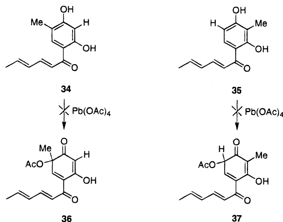
Scheme 9. Abortive Attempts To Prepare Acetates 36 and 37 from Resorcinols 34 and 35
