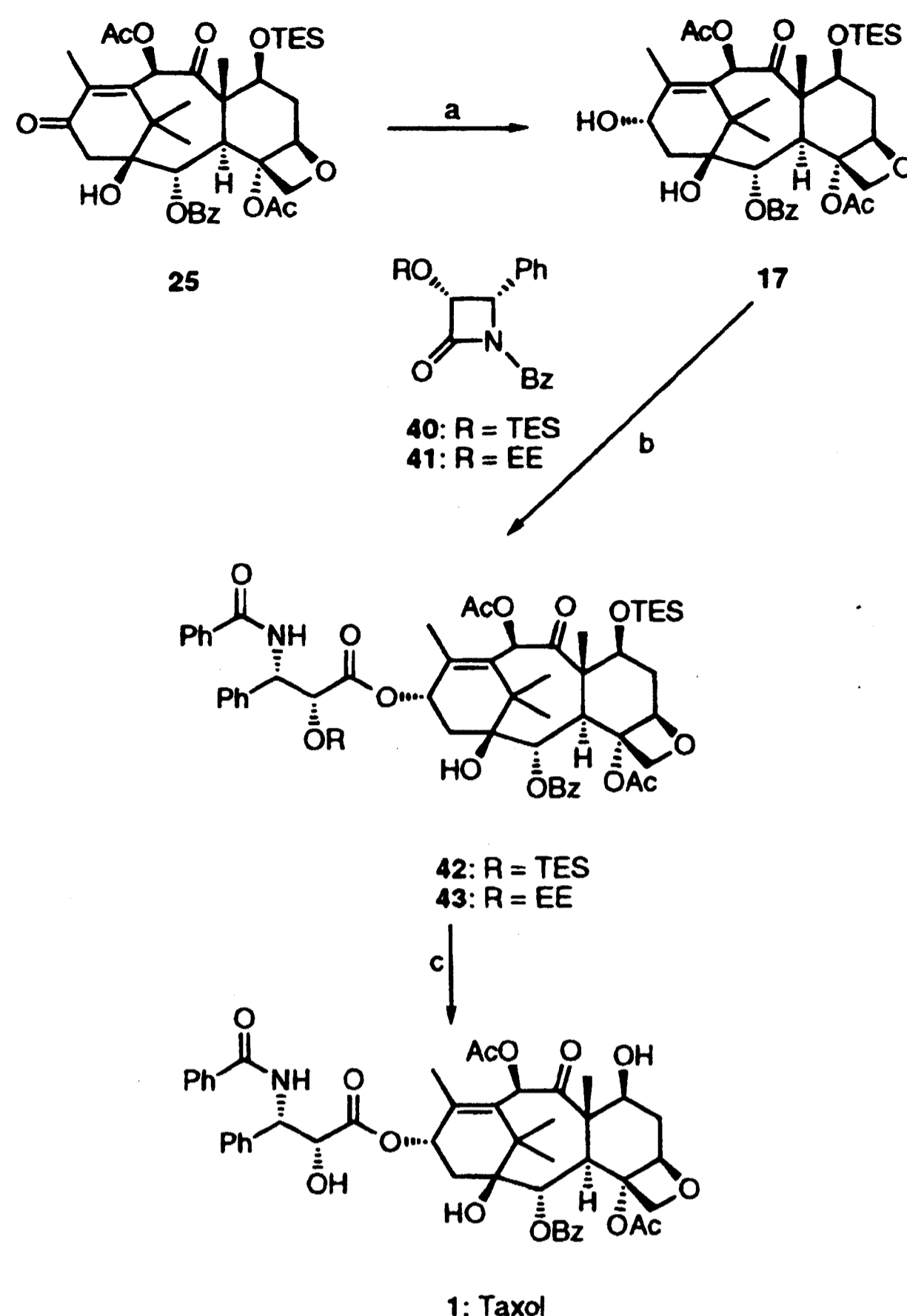
Scheme 8. Taxol's Side-Chain Attachment a
