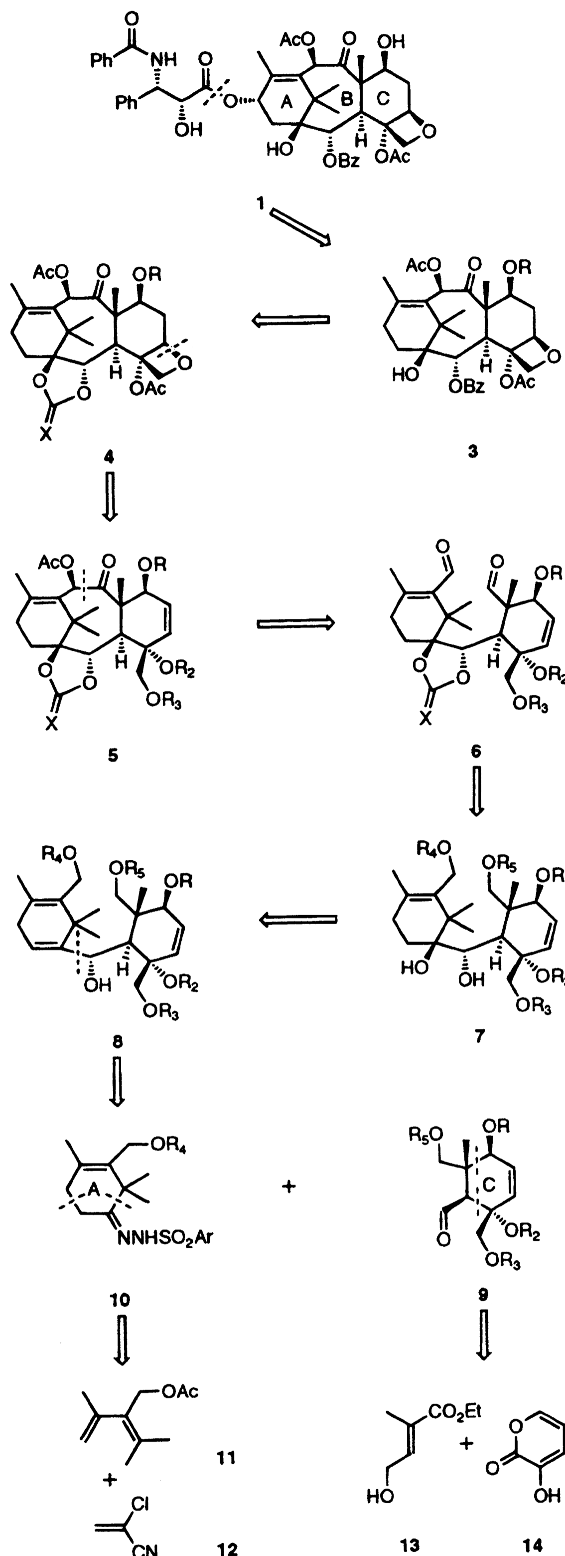
Scheme 1. Retrosynthetic Analysis of Taxol (1) a
