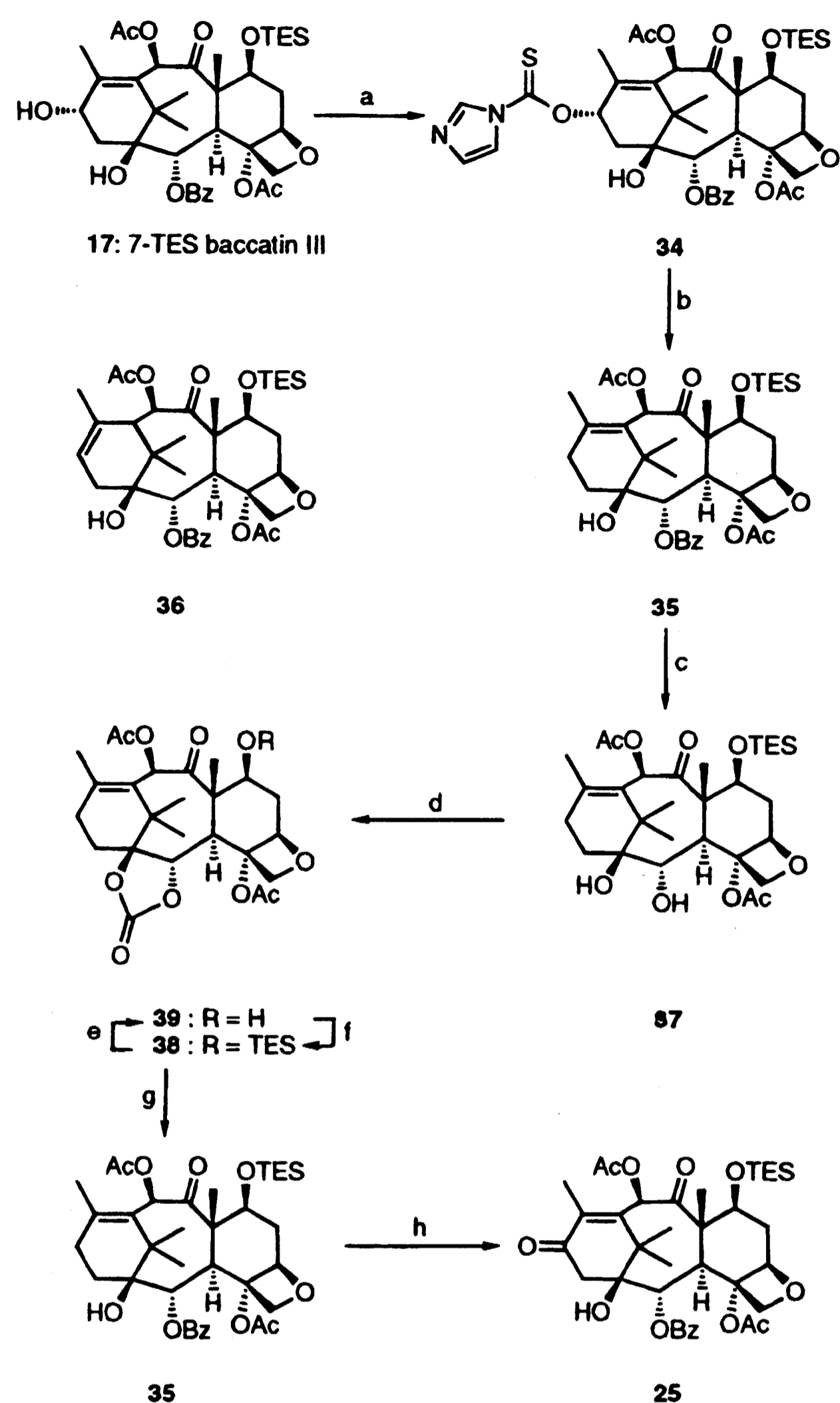
Scheme 7. C13 Deoxygenation and Oxygenation a
