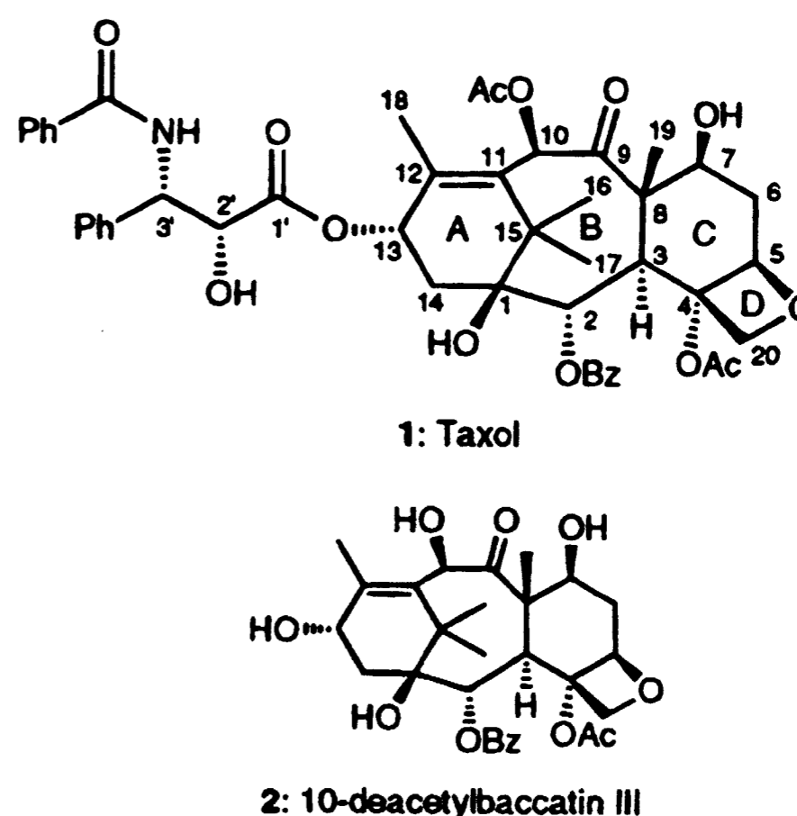
Figure 1. Structure of Taxol (1) and 10-deacetylbaccatin III (2).
